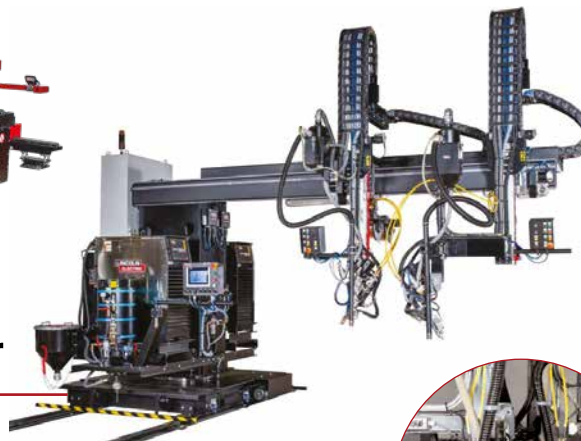
Beam welder
