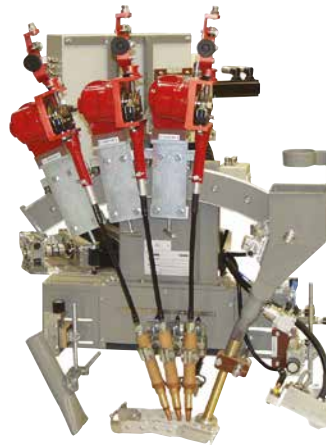
3arc welding head
