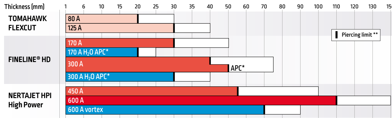
Plasma thickness range multi material
