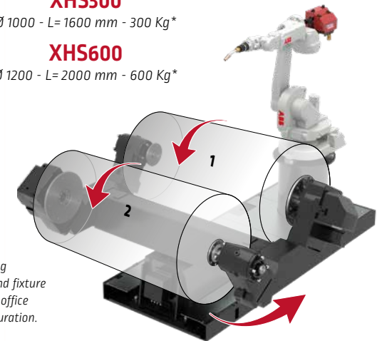
1 rotating table with 2 headstocks for 2 work envelopes.
