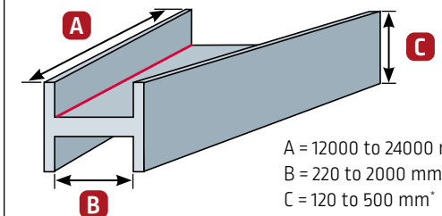
Standard / Dimensions for clamping bench
